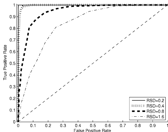
Fig. 3 ROC curve showing the ability of the proposed algorithm to accurately discover genes with an underlying time-dependent pattern with random noise at several relative standard deviations (RSD). RSD=0.2, AUROC=1; RSD=0.4, AUROC=0.995; RSD=0.8, AUROC=0.944; RSD=1.6, AUROC=0.839. The dashed diagonal line represent the parity line.
